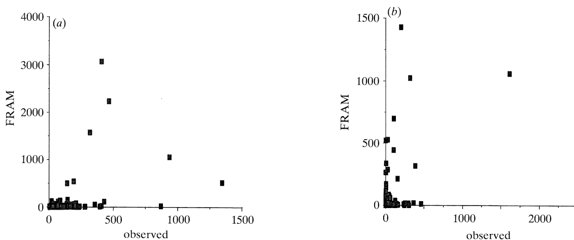
Figure 4. Scatterplot of observed current meter estimates of (a) EKE and (b) MKE , shown against the nearest FRAM grid point estimate. Units are \text{cm}^2 \text{ s}^{-2} .
