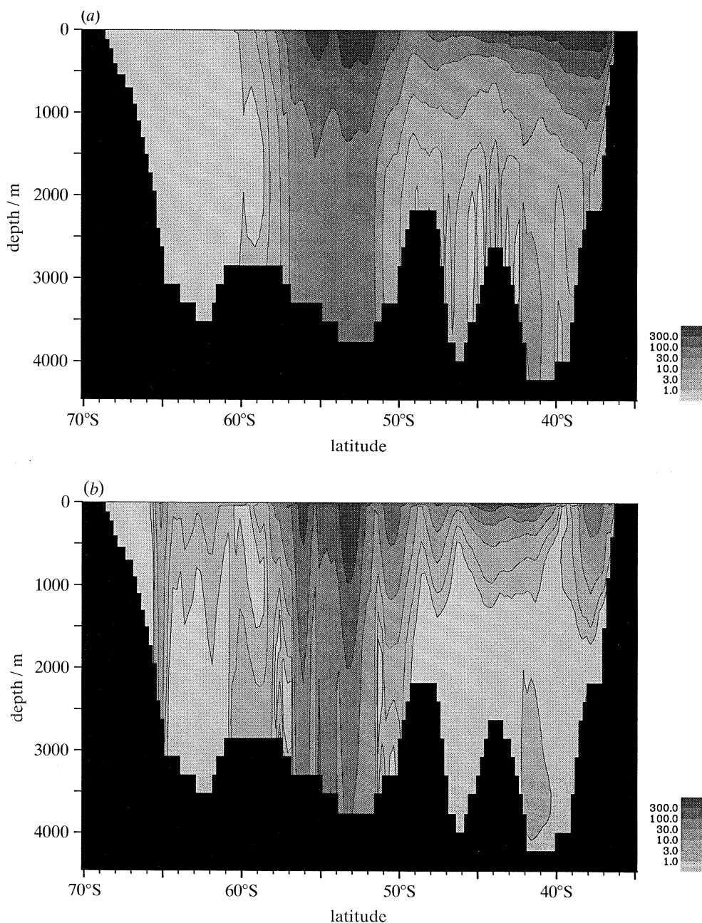
Figure 2. A section of (a) EKE and (b) MKE at 150°E in FRAM. Contour intervals 1, 3, 10, 30, 100 and 300 \text{cm}^2 \text{s}^{-1} .
