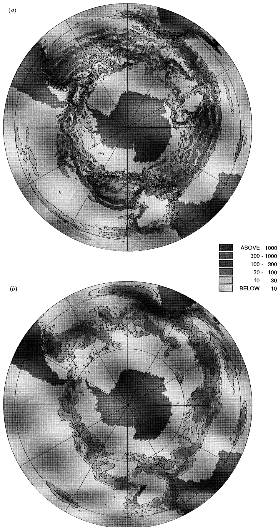
Figure 1. (a) The kinetic energy of the mean flow ( mKE ) at 32 m depth in FRAM. Contour intervals 10, 30, 100, 300 and 1000 \text{ cm}^2 \text{ s}^{-1} . (b) The mean eddy kinetic energy ( eKE ) at 32 m depth in FRAM. Contour intervals 10, 30, 100, 300 and 1000 \text{ cm}^2 \text{ s}^{-1} .
