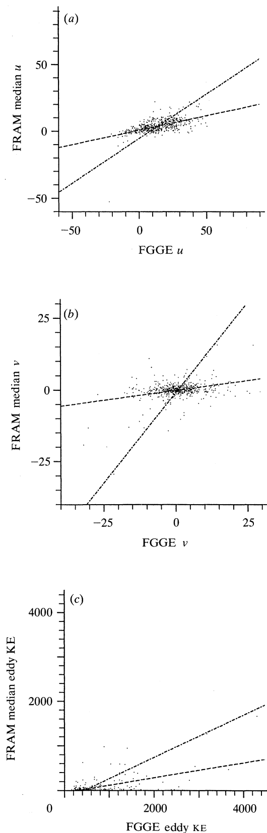
Figure 3. Correlations between FRAM data and FGGE drifter data at 32 m depth. Shown are (a) the mean eastward velocity; (b) the mean northward velocity; and (c) the EKE. The FRAM values are all medians over the 5^\circ square used to compute the FGGE data. The dashed line shows the best linear fit of FRAM on FGGE; the dash-dotted line the reverse. The angle between these lines gives a visual indication of the strength of the correlation. Units are \text{cm s}^{-1} .
